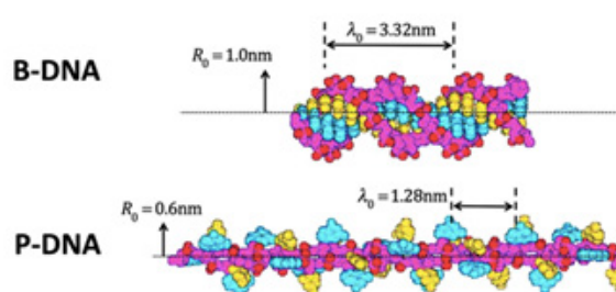
Figure 12: Two forms of DNA. Modified (2019) from Fig. 5 of Allemand et al. Proc. Natl. Acad. Sci. USA 95, 14152-14157 (1998), CC BY
