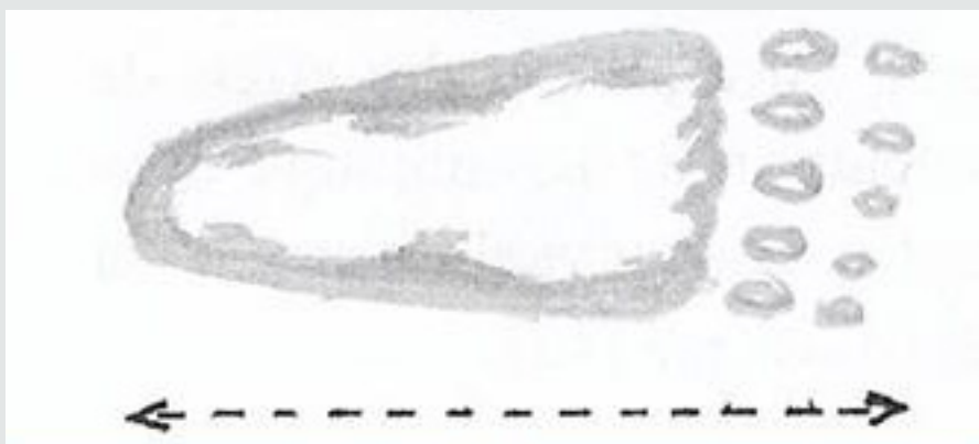
Figure 2: It Is Not About A Measure of Length.
