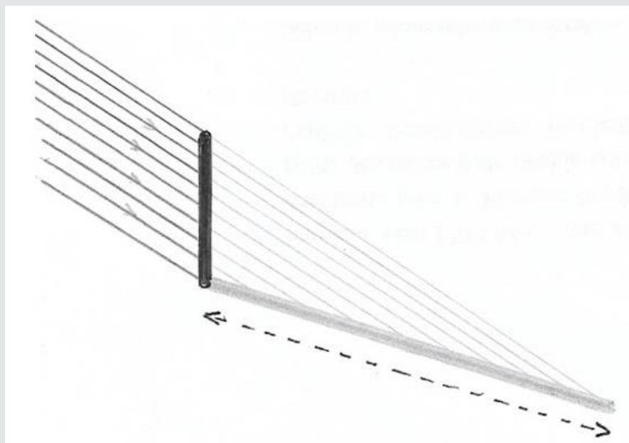
Figure 4: Eratosthenes Did Not Measure the Length.
