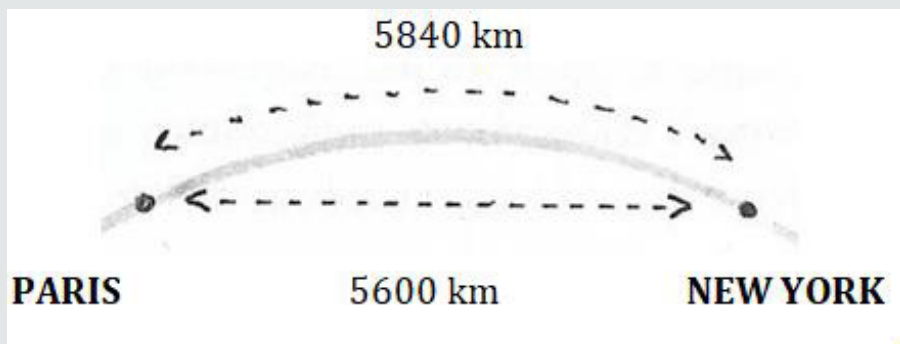
Figure 3: Physical Distance & Mathematical Distance.
