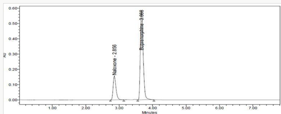
Figure 5: Standard Chromatogram of NAH and BUH.
