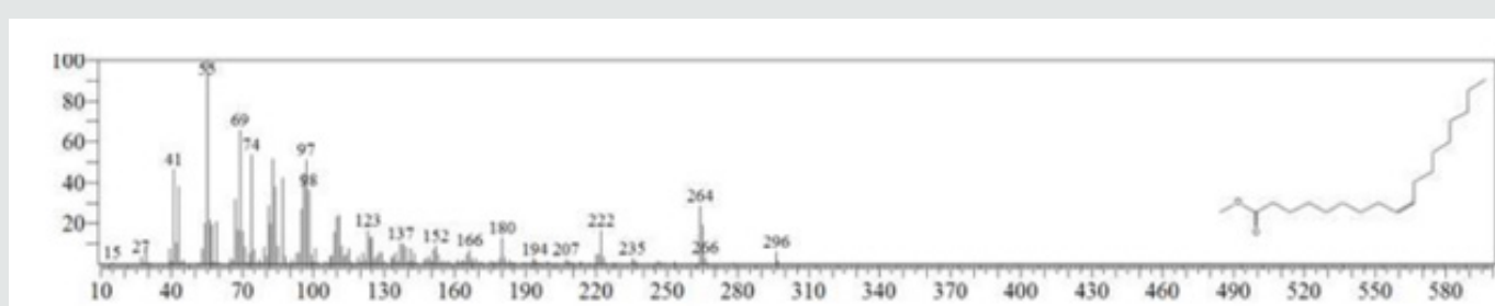
Figure 2: The Mass spectrum of 9-Octadecenoic acid (Z)-, methyl ester.
