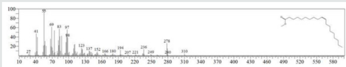
Figure 11: The Mass spectrum of cis-10-Nonadecenoic acid, methyl ester.
