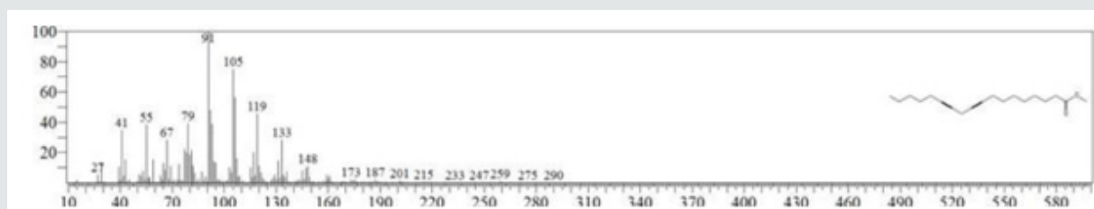
Figure 4: The Mass spectrum of 9,12-Octadecadiynoic acid, methyl ester.
