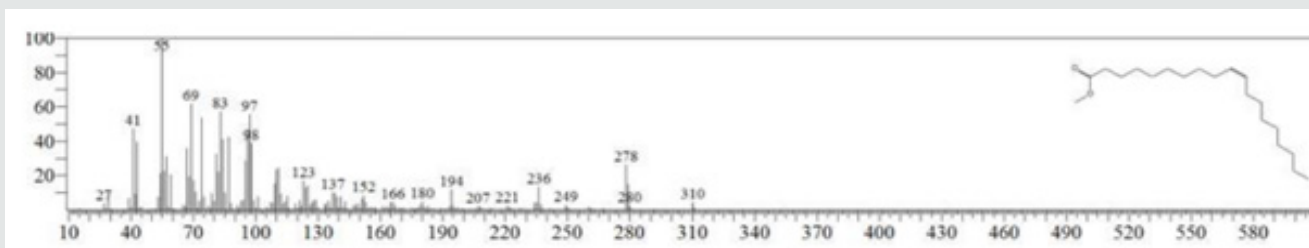
Figure 7: The Mass spectrum of 10-Nonadecenoic acid, methyl ester.
