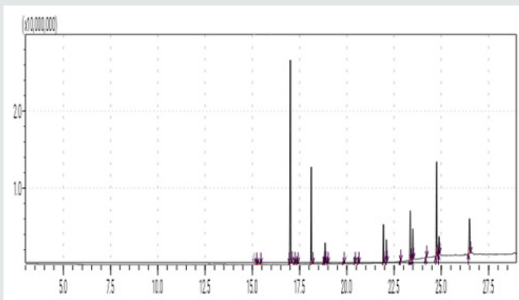
Figure 1: The typical GC chromatogram of Ximenia americana L seeds oil.
