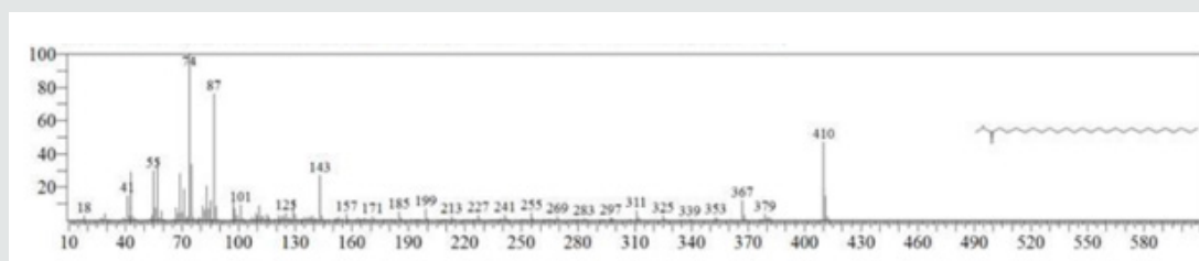
Figure 8: The Mass spectrum of Hexacosanoic acid, methyl ester.
