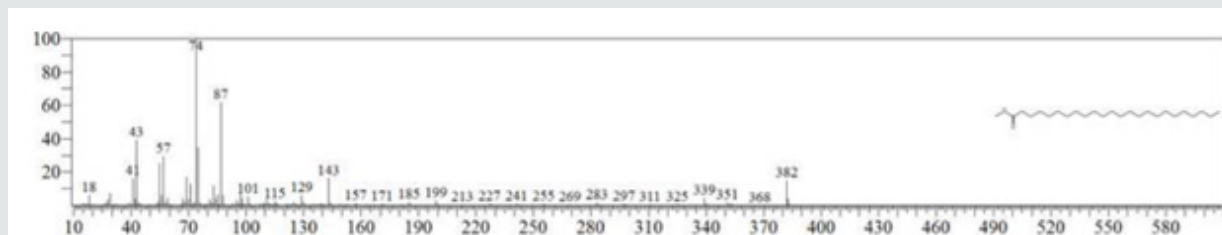
Figure 6: The Mass spectrum of Tetracosanoic acid, methyl ester.
