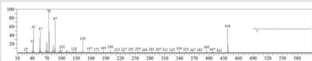
Figure 10: The Mass spectrum of Octacosanoic acid, methyl ester.
