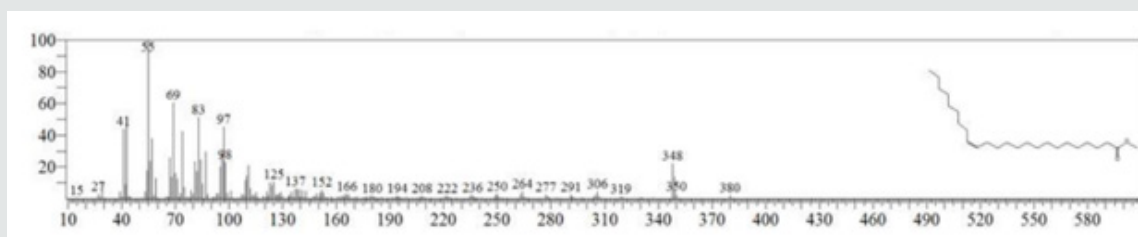
Figure 5: The Mass spectrum of 15-Tetracosenoic acid, methyl ester, (Z).
