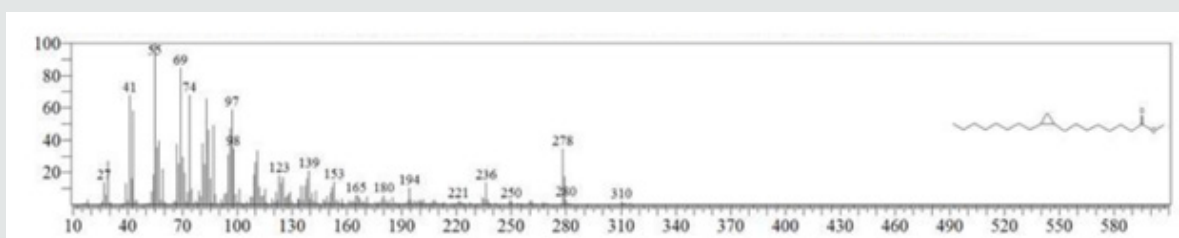
Figure 9: The Mass spectrum of Cyclopropanoic acid, 2-octyl-, methyl ester.
