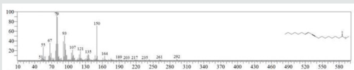
Figure 3: The Mass spectrum of Methyl octadeca-9-yn-11-trans-enoate.
