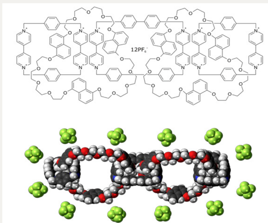
Figure 2: Molecular structure of Olympiadane Nano molecules.
