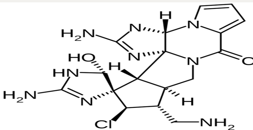
Figure 1: Molecular structure of Palau'amine Nano molecules.
