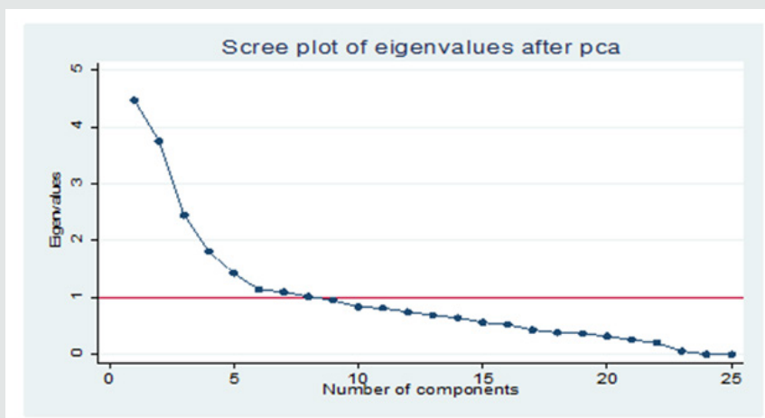
Figure 1: Scree plot of Eigen values after PCA.
