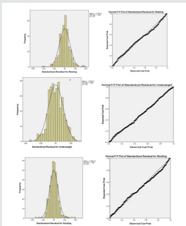
Figure 2: Histogram and p-p plots for Checking Model Adequacy of Multivariate Multiple Linear Regression for Overall Sample Data.
